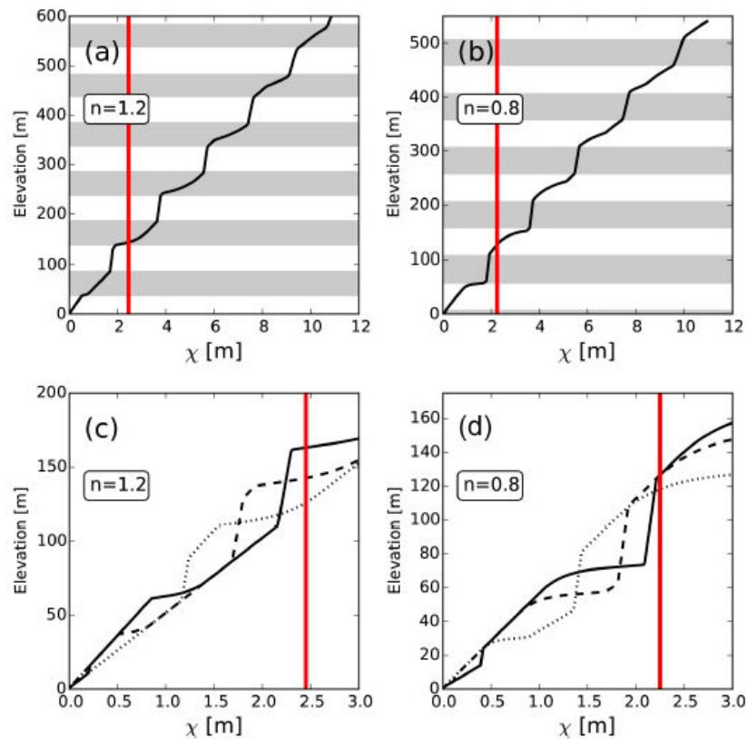
Figure 9. Simulations of knickpoint propagation and damping from base level. Entire equilibrium profiles are depicted for cases where n = 1.2 (a) and n = 0.8 (b). Panels (c) and (d) show zoomed-in figures that depict three separate time steps (dotted, dashed, and then solid) as fast knickpoints catch up with slow knickpoints at the calculated damping length scale ( \lambda , thick red line). The interaction of the two knickpoints can be visualized as the reduction in size of a slope patches that are at the topographic equilibrium slope as these patches approach \lambda
