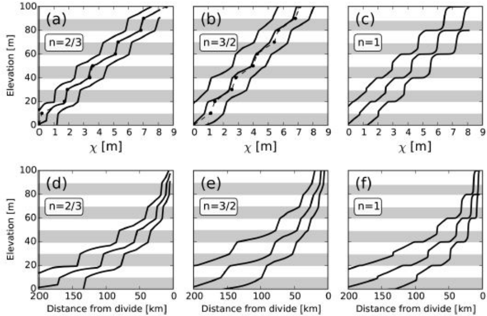
Figure 5. Channel profiles in subhorizontally layered rocks with low uplift ( 0.25 \text{ mmyr}^{-1} ). (a-c) Channel profiles in x-elevation space for cases where n = 2/3 (a), n = 3/2 (b), and n = 1 (c). (d-f) Channel profiles as a function of distance from divide. Grey bands indicate weaker rocks. The low-uplift simulations utilize longer distances and thinner rock layers in order to obtain a similar number of rock layer cycles. These profile shapes are qualitatively similar to the high-uplift cases (Fig. 4).
