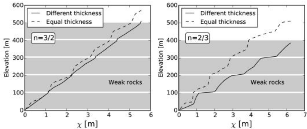
Figure 7. The influence of relative layer thickness on slopes in continuity steady state. If the relative thickness of the strong and weak layers is changed, the slopes that are far from base level in both rocks adjust correspondingly (solid lines), as predicted by continuity steady state. Grey bands depict the locations of weak rocks in the differing thickness model. The dashed lines depict channel profiles for simulations with equal layer thickness but the same erosional parameters. Increasing the weak layer percentage reduces topography overall.
