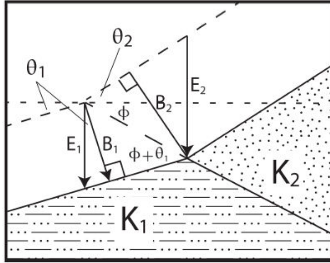
Figure A1. Geometric relationships used to derive the equation for continuity of the channel at a contact between two rock types. Note that the slope of the contact plane ( S_c = \tan \phi ) is defined as positive when the contact dips in the downstream direction.
