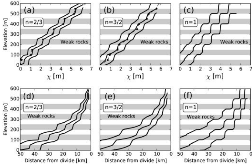
Figure 4. Channel profiles in subhorizontally layered rocks with high uplift ( 2.5 \text{ mmyr}^{-1} ). (a-c) Channel profiles in \chi -elevation space for cases where n = 2/3 (a), n = 3/2 (b), and n = 1 (c). (d-f) Channel profiles as a function of distance from divide. Each panel contains three time snapshots of the profile with uplift subtracted from elevation so that the profiles evolve from left to right. Grey bands represent the weak rock layers. The dashed lines (a, b) show the profiles predicted by the continuity steady-state theory (Eqs. 5 and 8), with filled circles depicting predicted crossing points of the contacts. Channel profiles obtain a steady-state shape except near base level, where a constant rate of base-level fall is imposed. For n \neq 1 the equilibrium profile steepness (slope in \chi space) has a one-to-one relationship with rock erodibility, with steeper channels in weaker rock if n < 1 . For n = 1 there is no unique relationship between erodibility and steepness, as continuity cannot be maintained along the entire profile (Matija Perne et al,2017)
