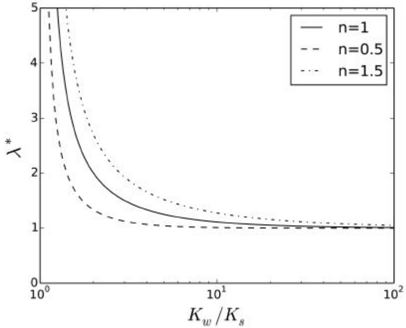
Figure 8. The dimensionless damping length scale, \lambda^* , as a function of erodibility ratio. Damping of base-level perturbations is strong when the erodibility ratio is greater than 3. \lambda^* can be interpreted as roughly the number of pairs of strong and weak rock layers that base-level perturbations must pass through before substantial damping toward continuity steady state.
