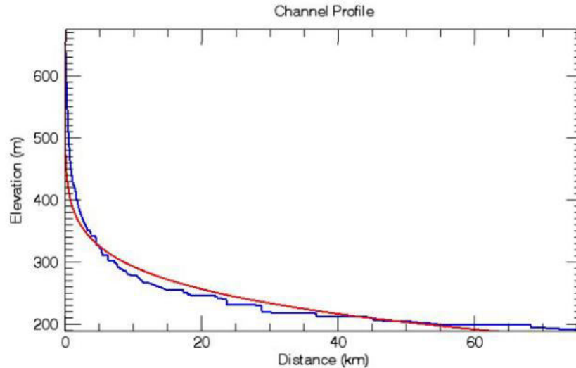
Figure. 2. Best fit of power-laws (9) and (22) to the main channel profile of the Nagduari Rift. Standard error = 15.93 and p = 0.133 .
