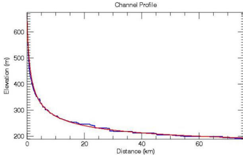
Figure. 1. Best fit of (4) to the main channel profile of Beaver Creek, KY.
